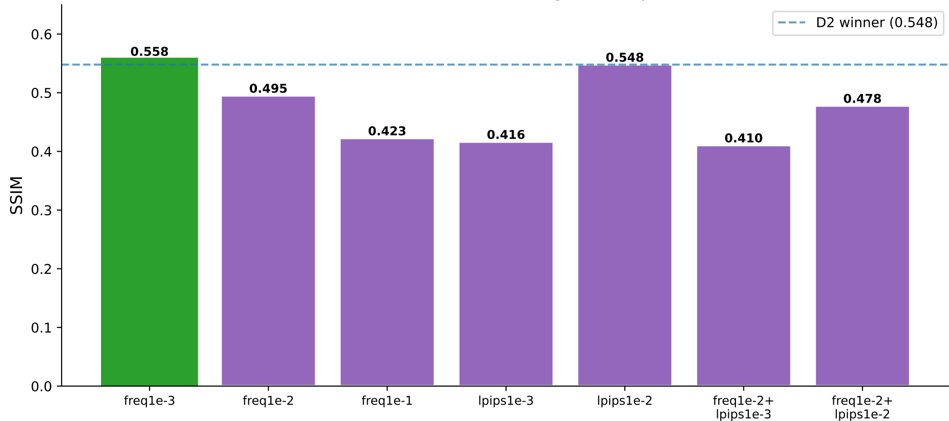
D3v2 — Frequency & Perceptual Prior Ablation (baseline: D2 winner config + extra prior)
