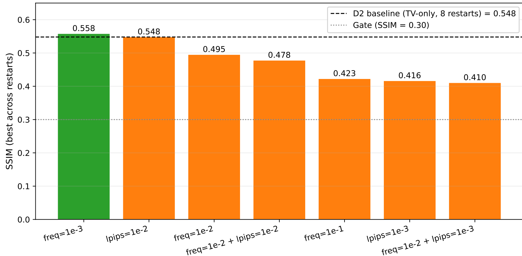
D3 image-prior ablation on Flowers102 (signAdam, tv=1e-1, lr=0.05, 30K iters, n_restarts=2)
