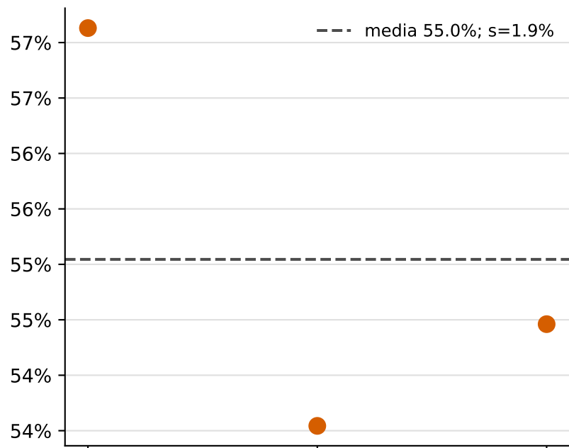
WER textual
