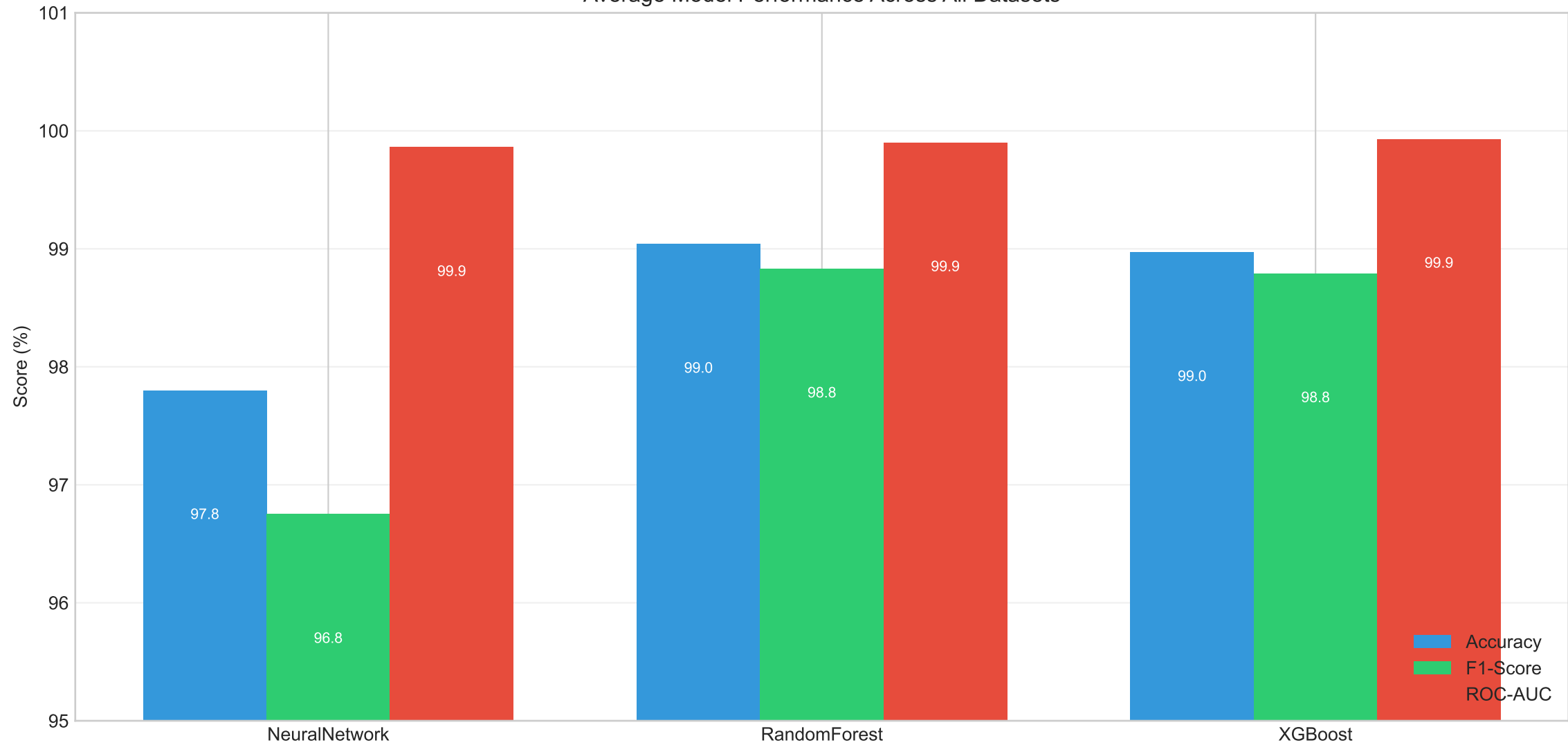
Average Model Performance Across All Datasets
