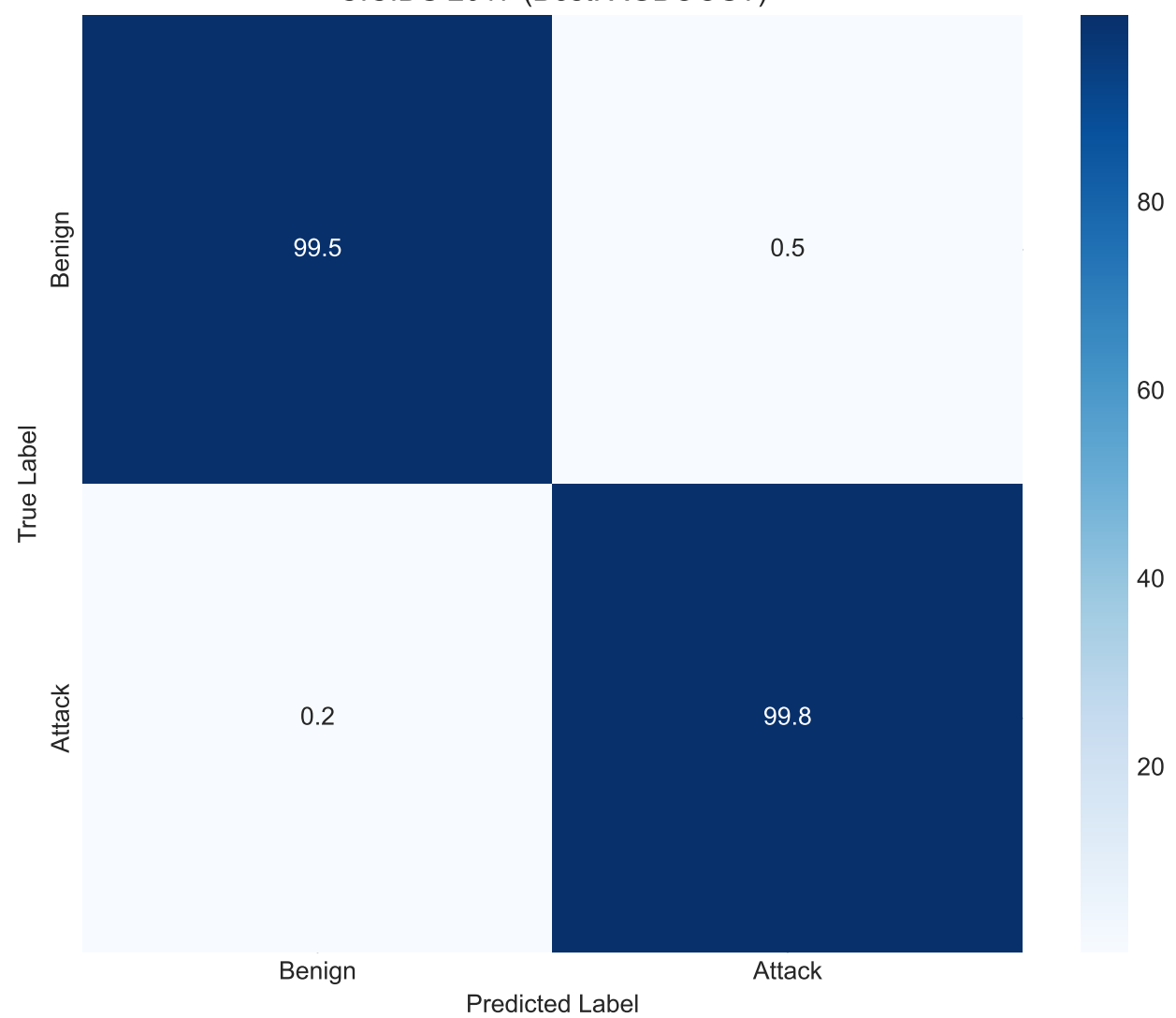
Zero-Day (Best: XGBOOST)
