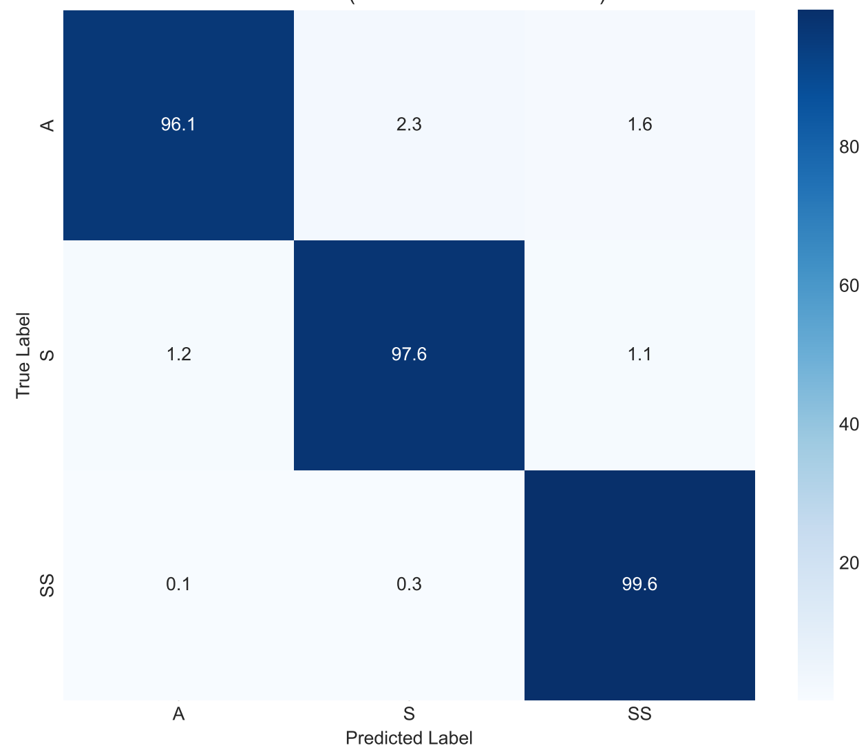
Ransomware (Best: RANDOMFOREST)
