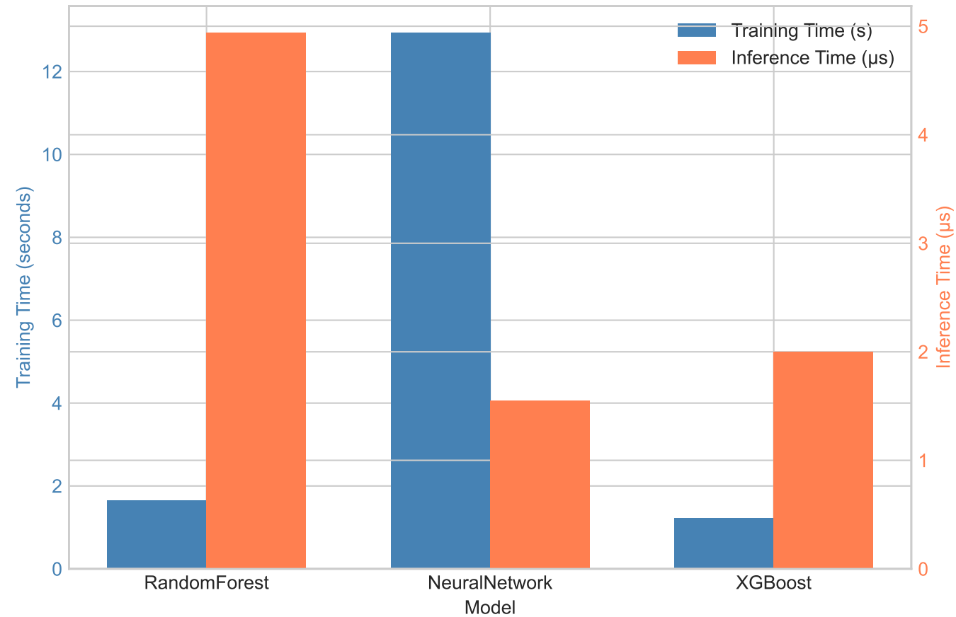
Training and Inference Time Comparison
