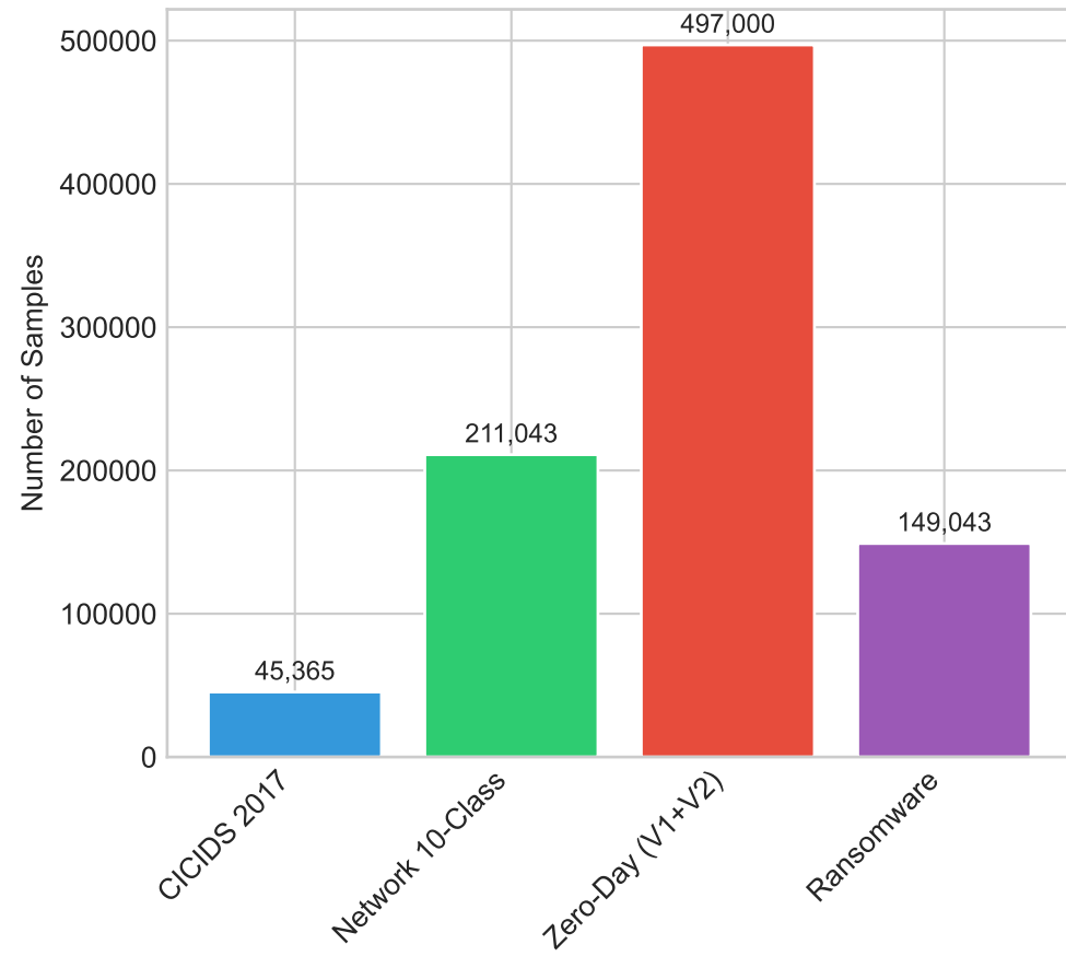
Dataset Size Comparison
