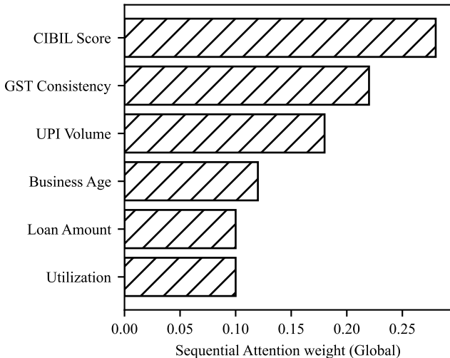
TabNet Feature Importance
