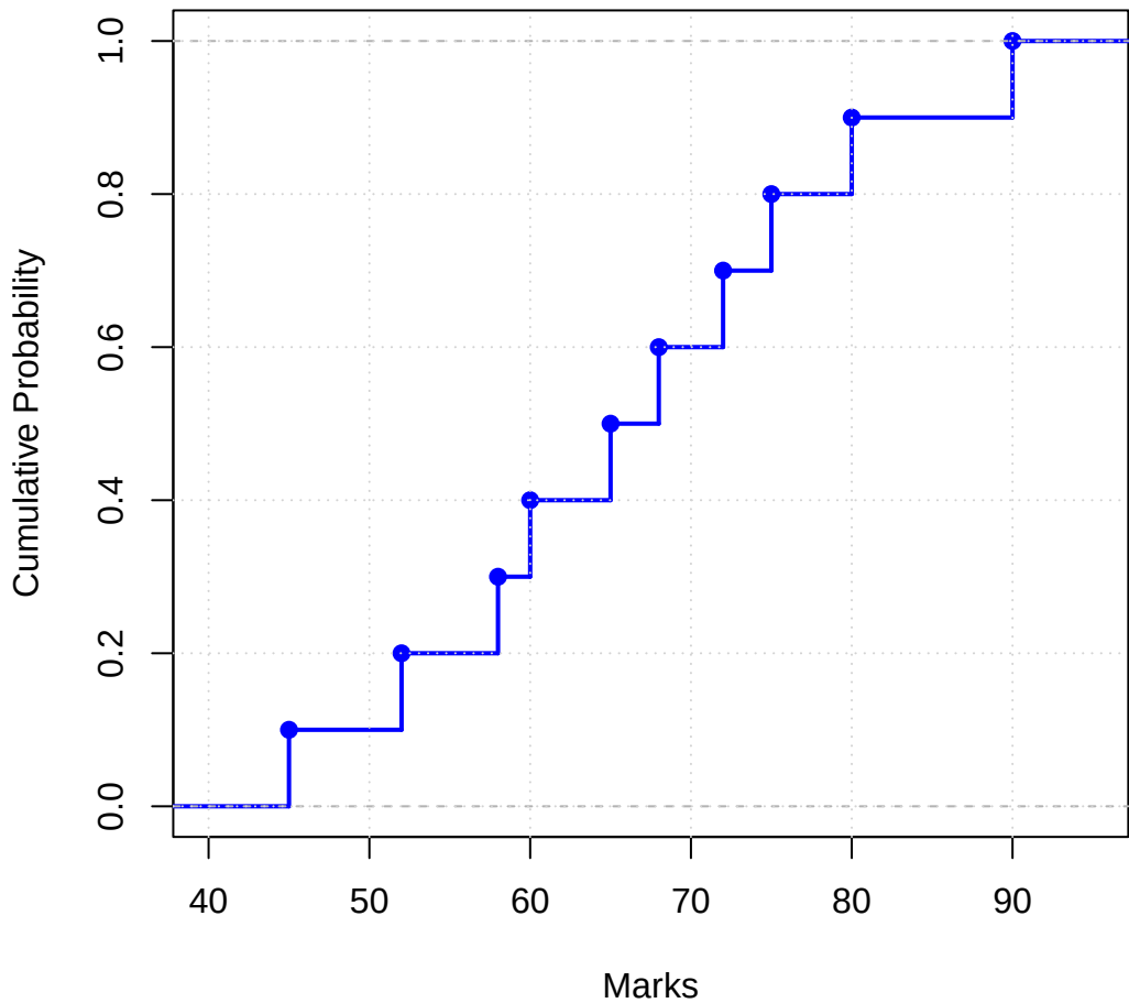
ECDF of Student Marks
