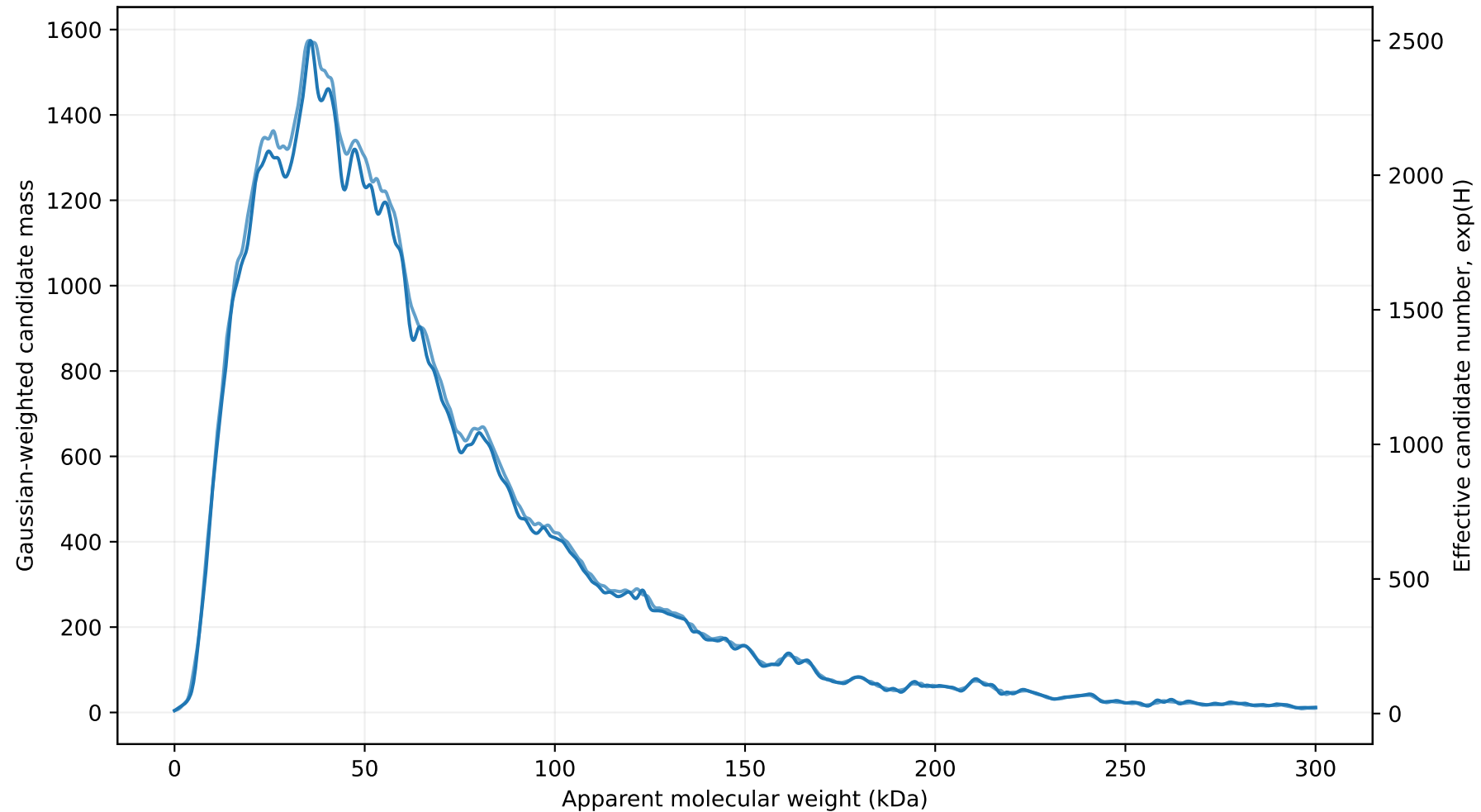
Molecular-weight identity ambiguity across the proteome
