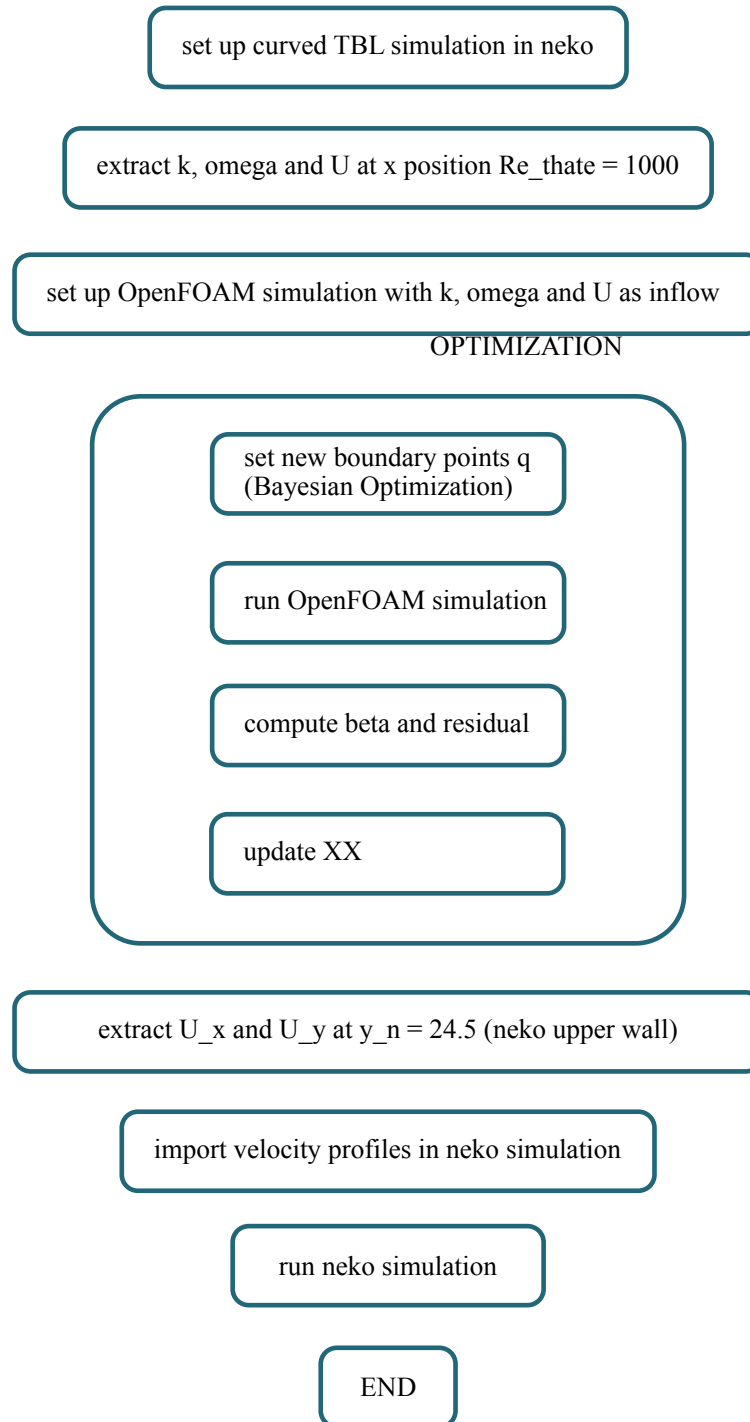
Figure 3.1: Worklow
