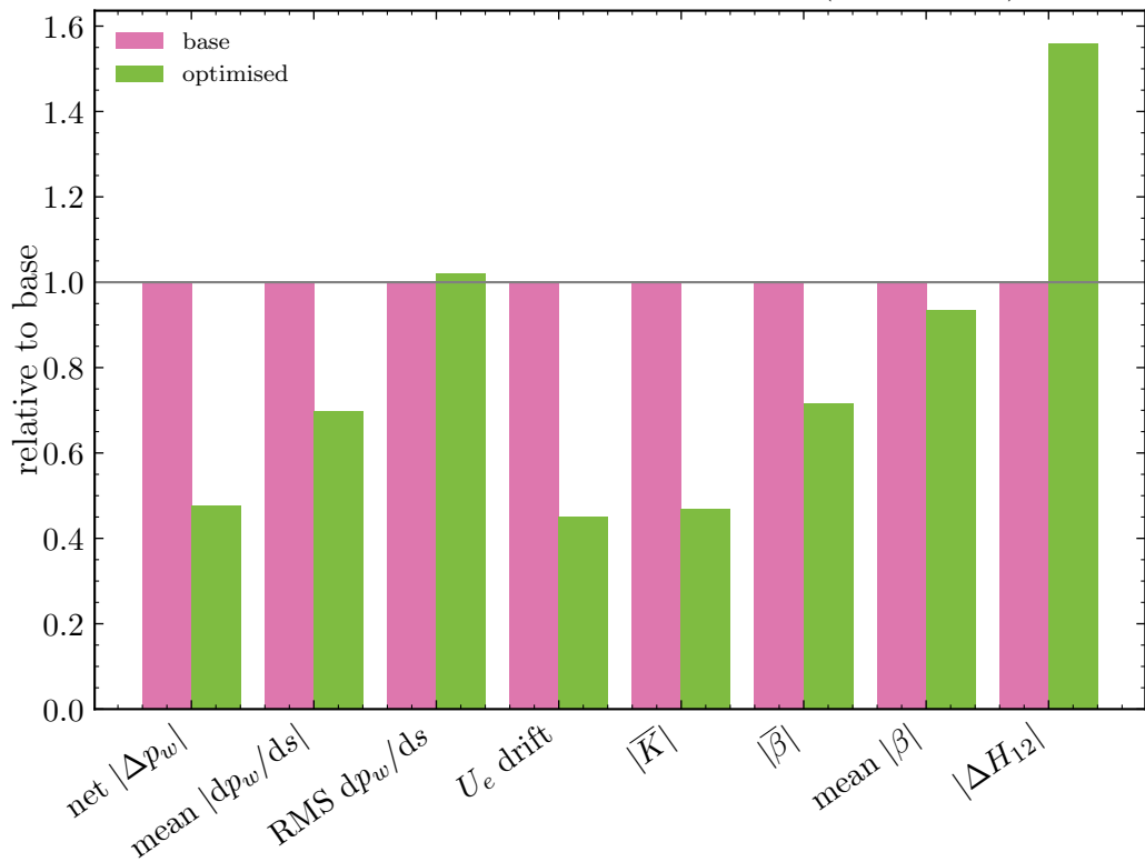
Pressure-gradient measures over the bend ( s = 335..634 )
