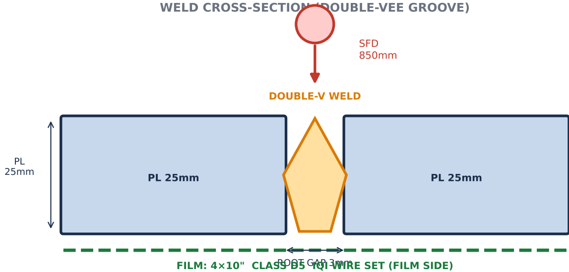
WELD CROSS-SECTION (DOUBLE-VEE GROOVE)
