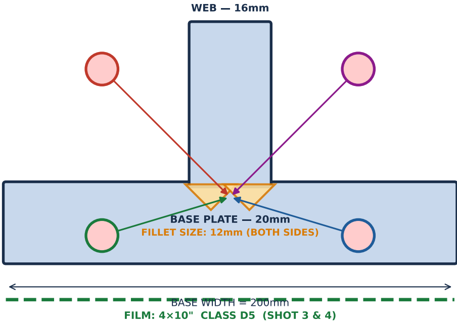
T-JOINT CROSS-SECTION (FILLET BOTH SIDES)
