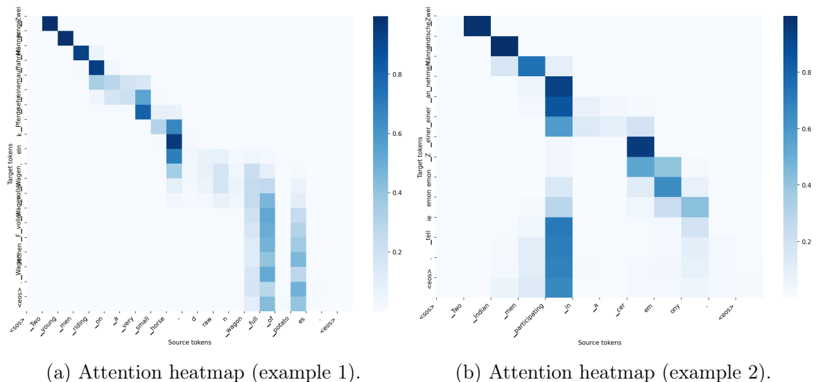
Figure 13: Attention alignments for the seq2seq model.
