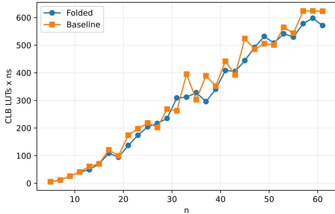
Area-Delay Product (ADP)
