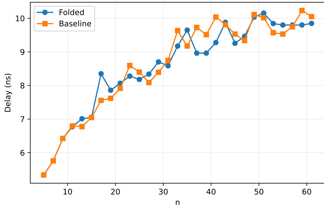
Vivado Datapath Delay
