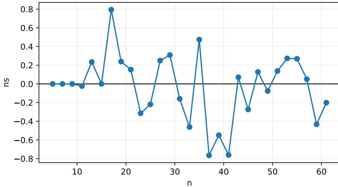
WNS Delta (B-F)
