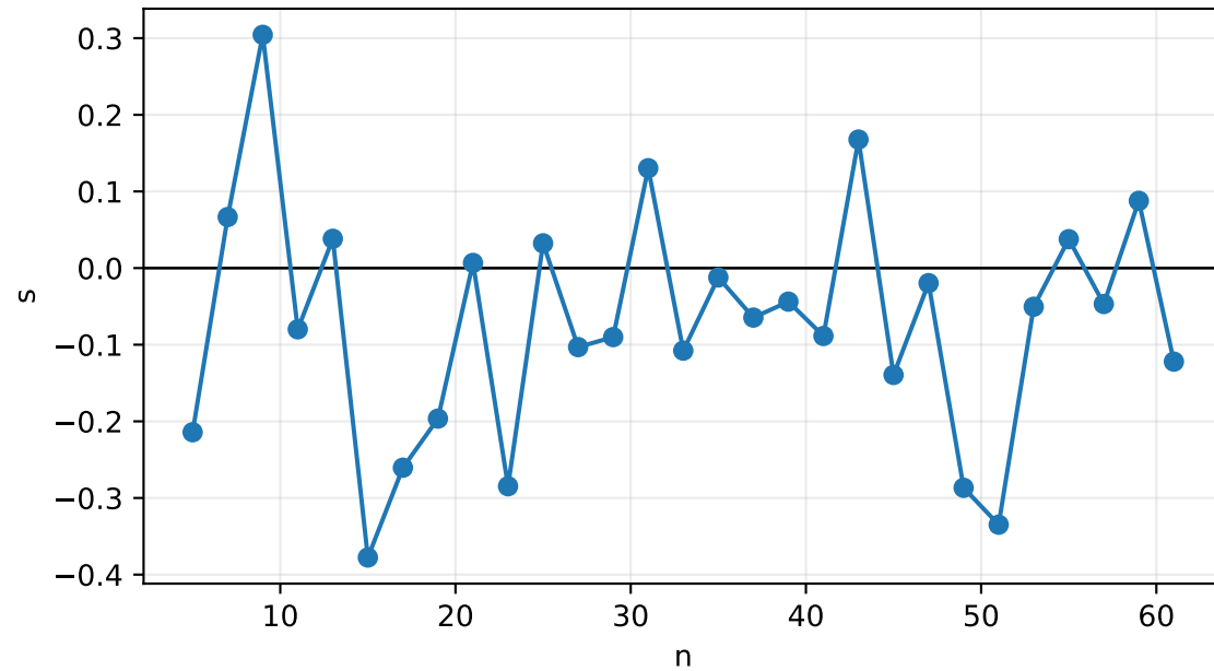
Runtime Delta (B-F)
