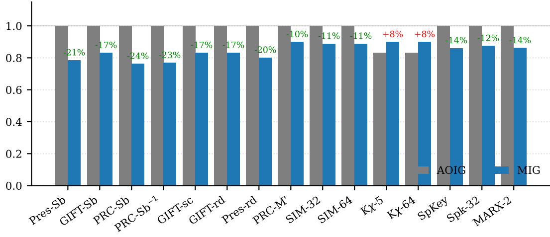
Per-vector fault detection prob
