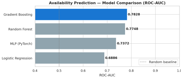
Fig. 5. Availability prediction model comparison by ROC-AUC. Gradient Boosting achieves the best score (0.783), followed by Random Forest (0.775), MLP (0.737), and Logistic Regression (0.689). All models outperform the random baseline (0.5).
