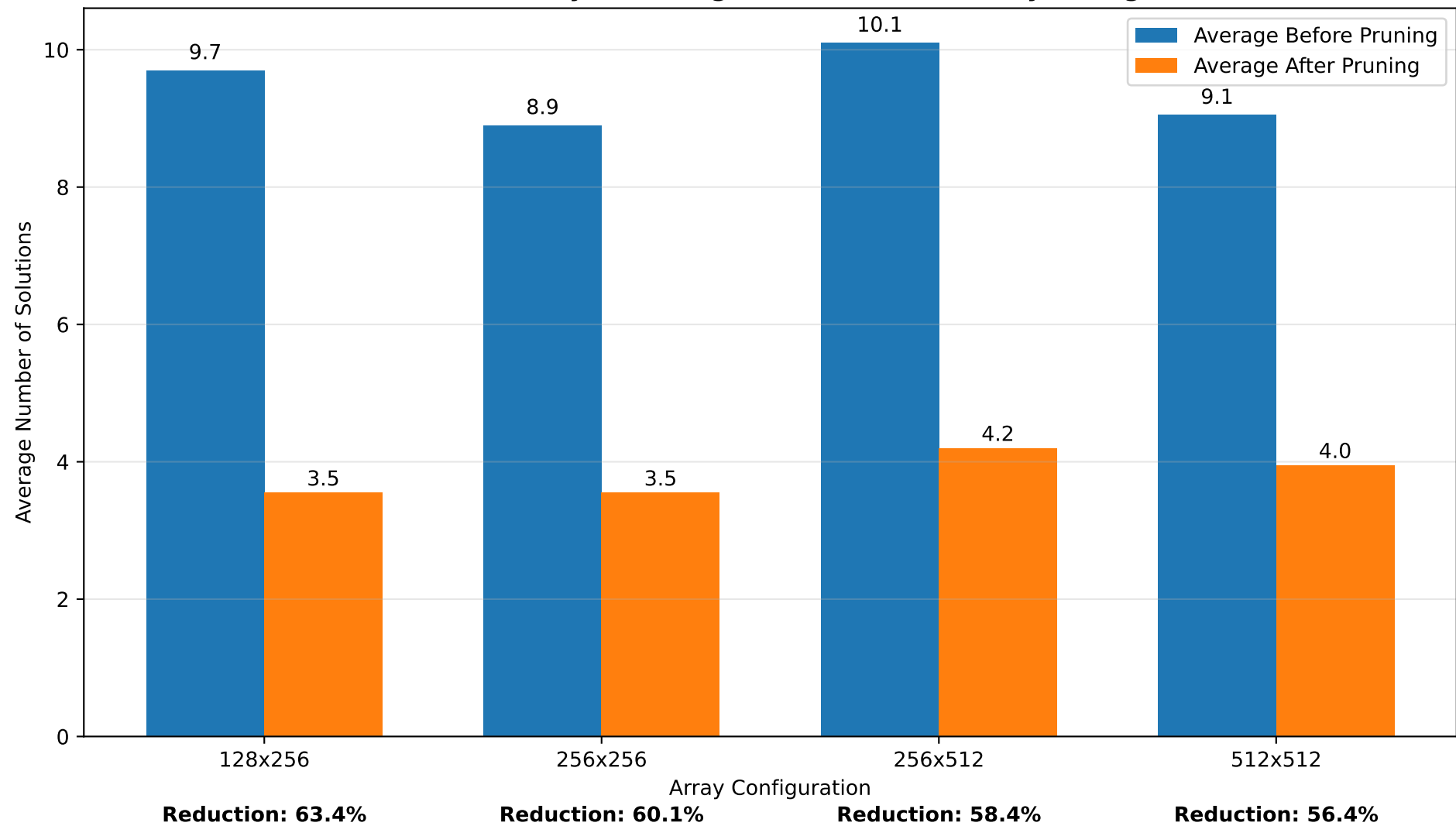
RESNET20 - Summary of Average Results Across Array Configurations
