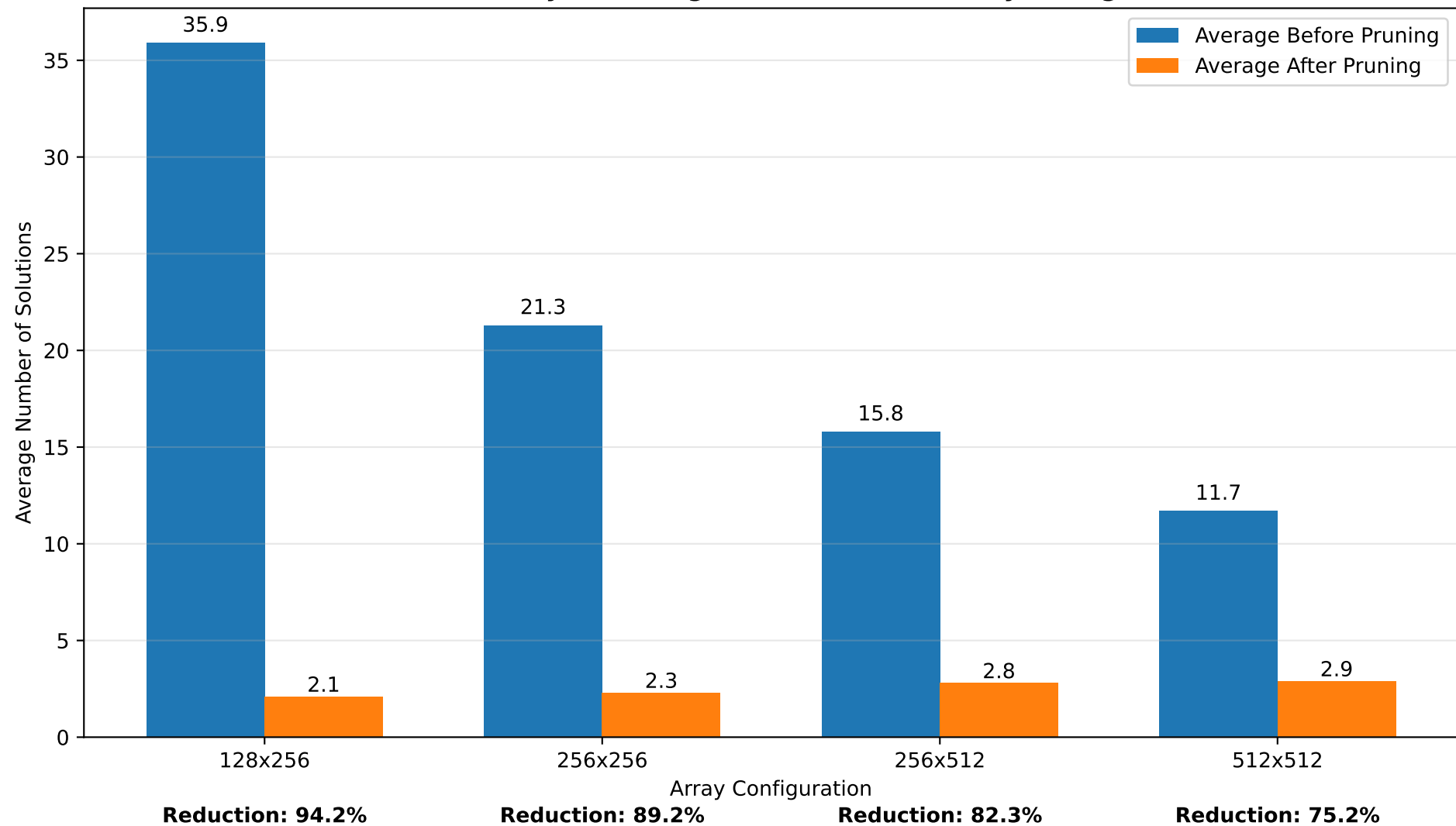
VGG16 - Summary of Average Results Across Array Configurations
