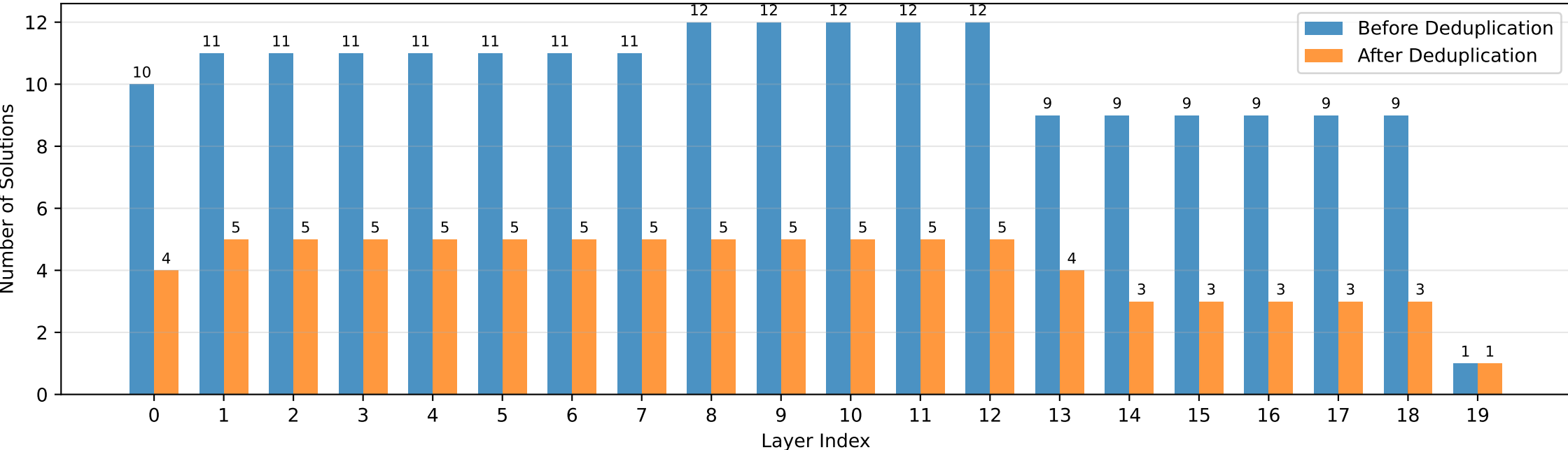
RESNET20 - Array 512x512
