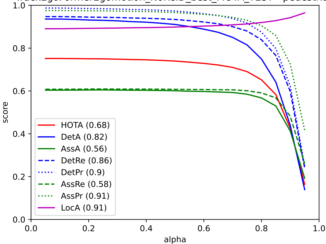
TrackEgoFormerEgomotion_NoReID_best_MOTA_TEST - pedestrian
