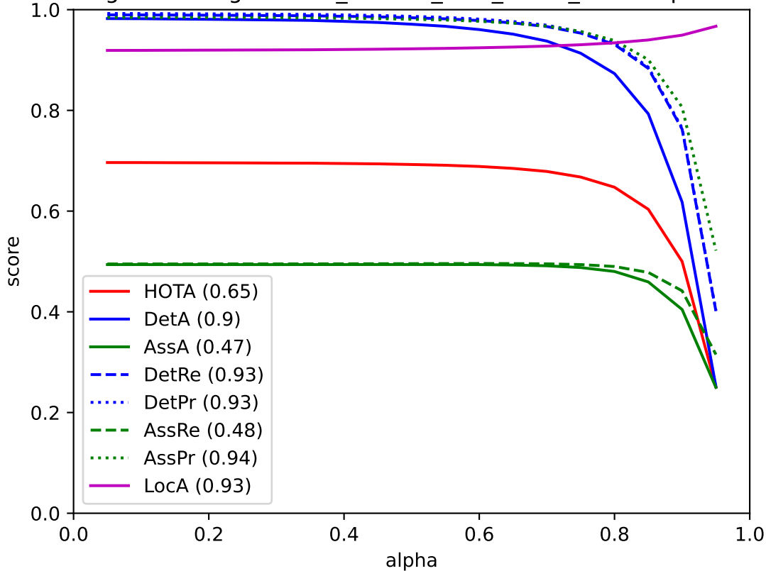
TrackEgoFormerEgomotion_NoReID_best_MOTA_TRAIN - pedestrian
