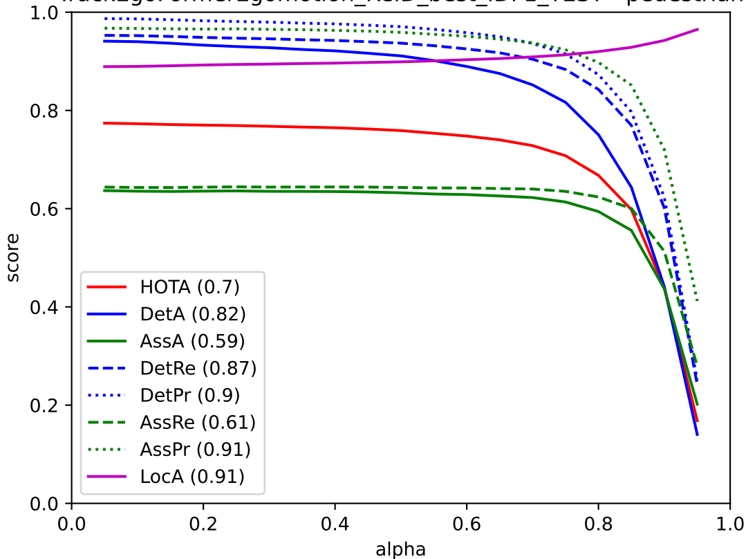
TrackEgoFormerEgomotion_ReID_best_IDF1_TEST - pedestrian
