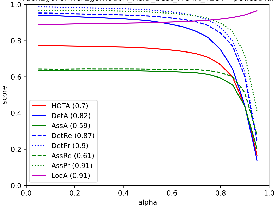
TrackEgoFormerEgomotion_ReID_best_MOTA_TEST - pedestrian
