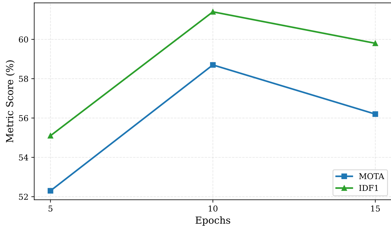
Validation Metric Trade-offs Over Epochs (egohumans_egomotion)
