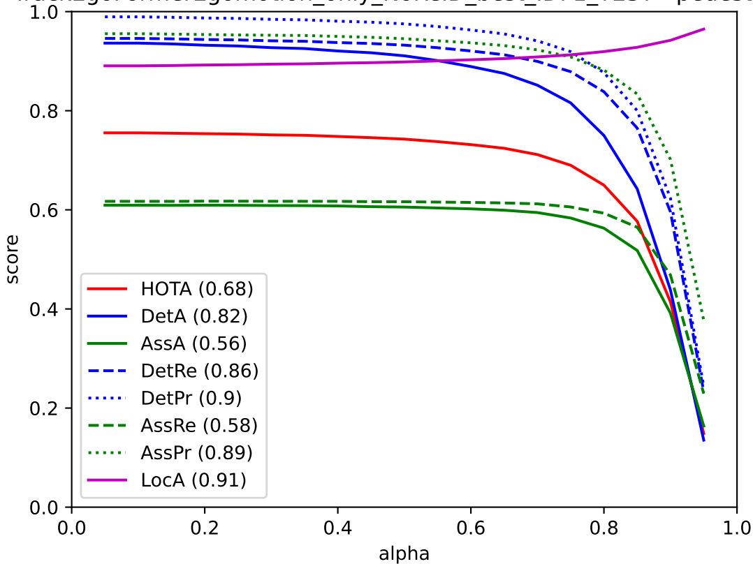
TrackEgoFormerEgomotion_only_NoReID_best_IDF1_TEST - pedestrian
