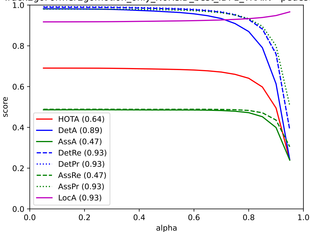
TrackEgoFormerEgomotion_only_NoReID_best_IDF1_TRAIN - pedestrian
