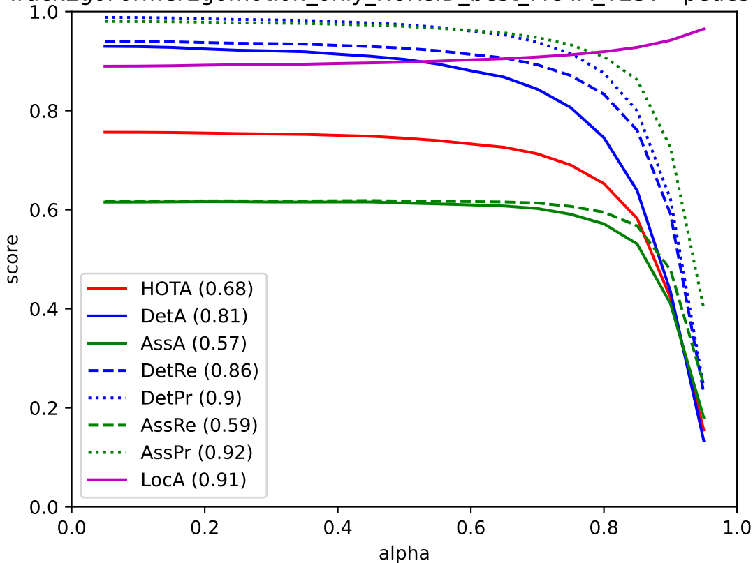
TrackEgoFormerEgomotion_only_NoReID_best_MOTA_TEST - pedestrian
