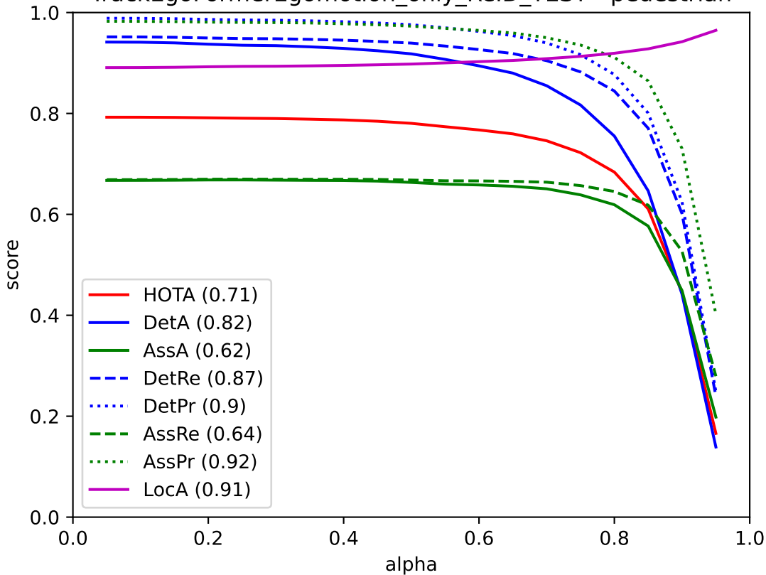
TrackEgoFormerEgomotion_only_ReID_TEST - pedestrian
