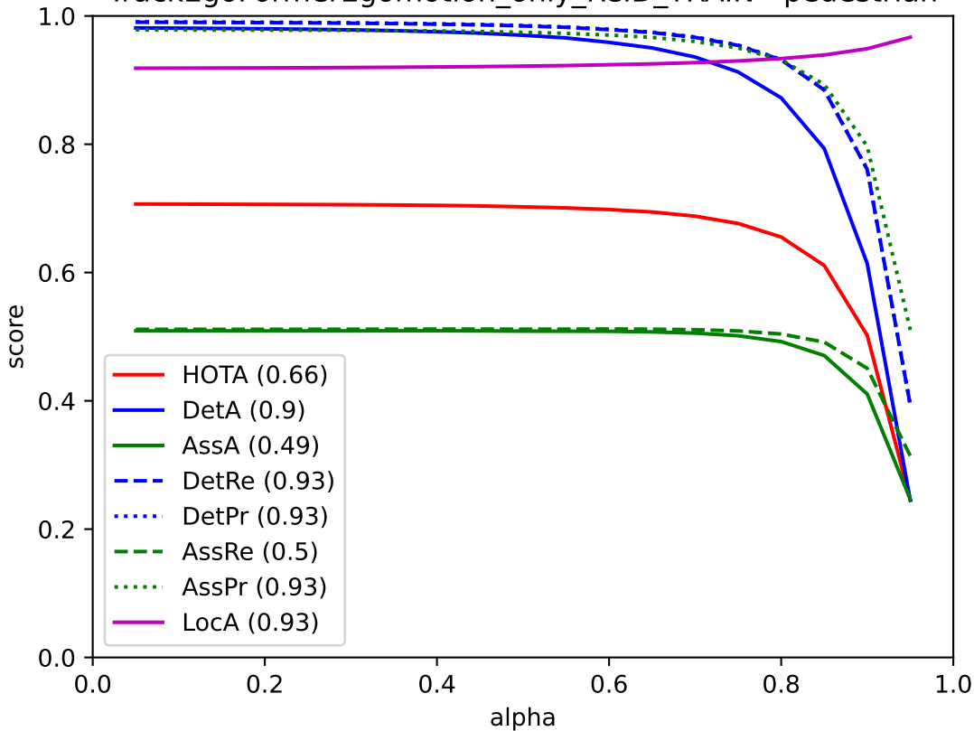
TrackEgoFormerEgomotion_only_ReID_TRAIN - pedestrian
