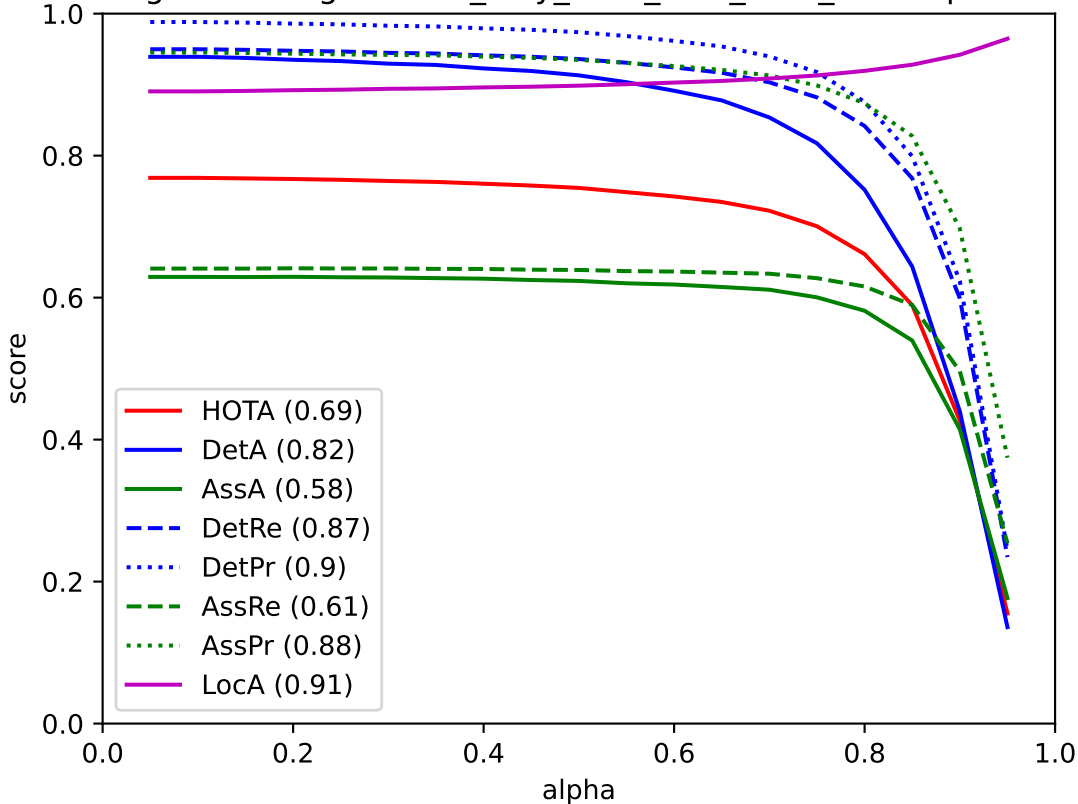
TrackEgoFormerEgomotion_only_ReID_best_IDF1_TEST - pedestrian
