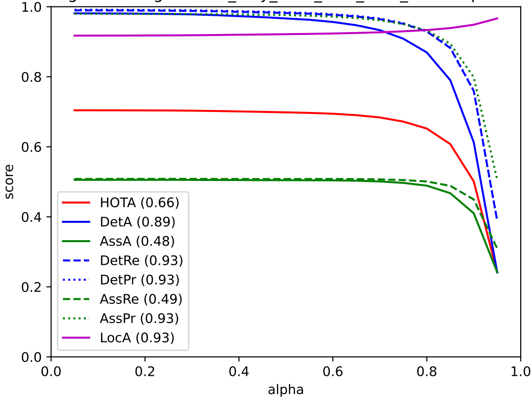
TrackEgoFormerEgomotion_only_ReID_best_IDF1_TRAIN - pedestrian
