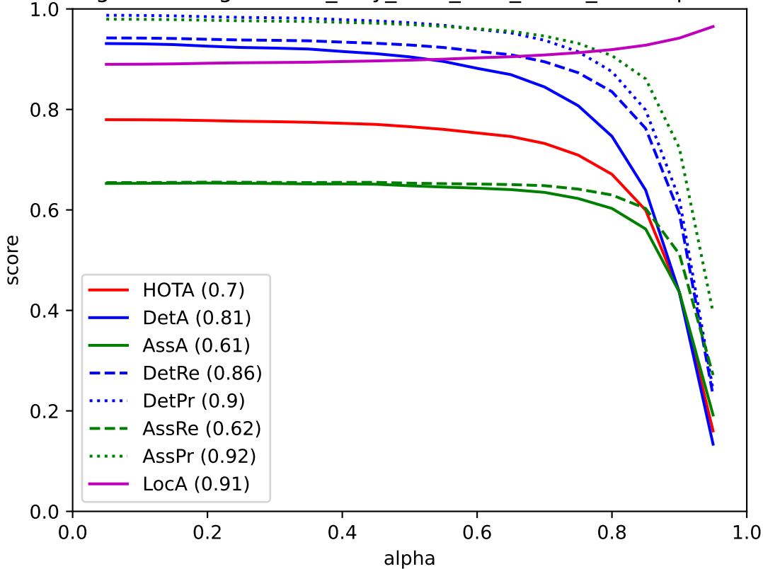
TrackEgoFormerEgomotion_only_ReID_best_MOTA_TEST - pedestrian
