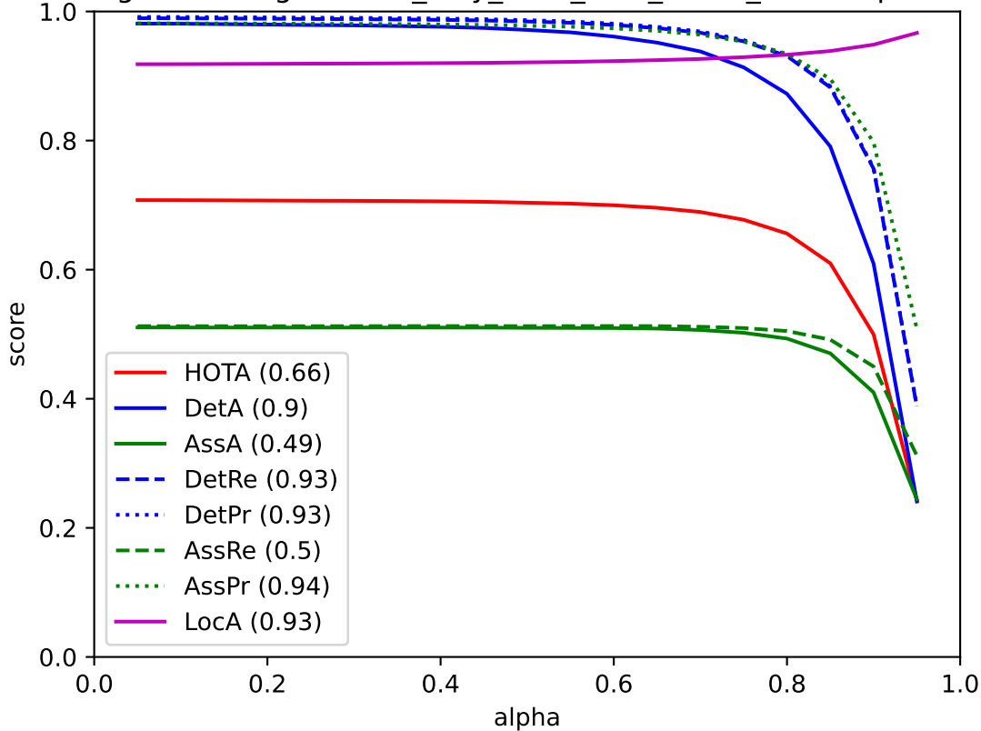
TrackEgoFormerEgomotion_only_ReID_best_MOTA_TRAIN - pedestrian
