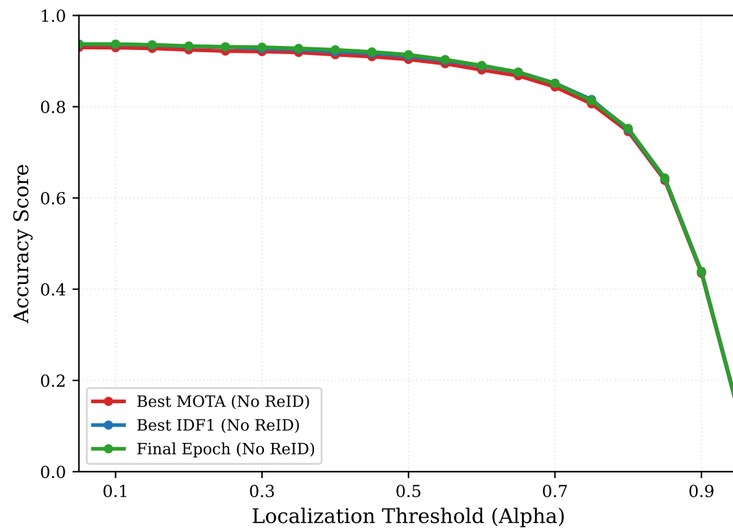
Detection Accuracy ( DetA Curve) - No ReID
