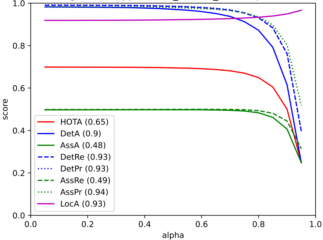
TrackEgoFormerAppearance NoReID TRAIN - pedestrian
