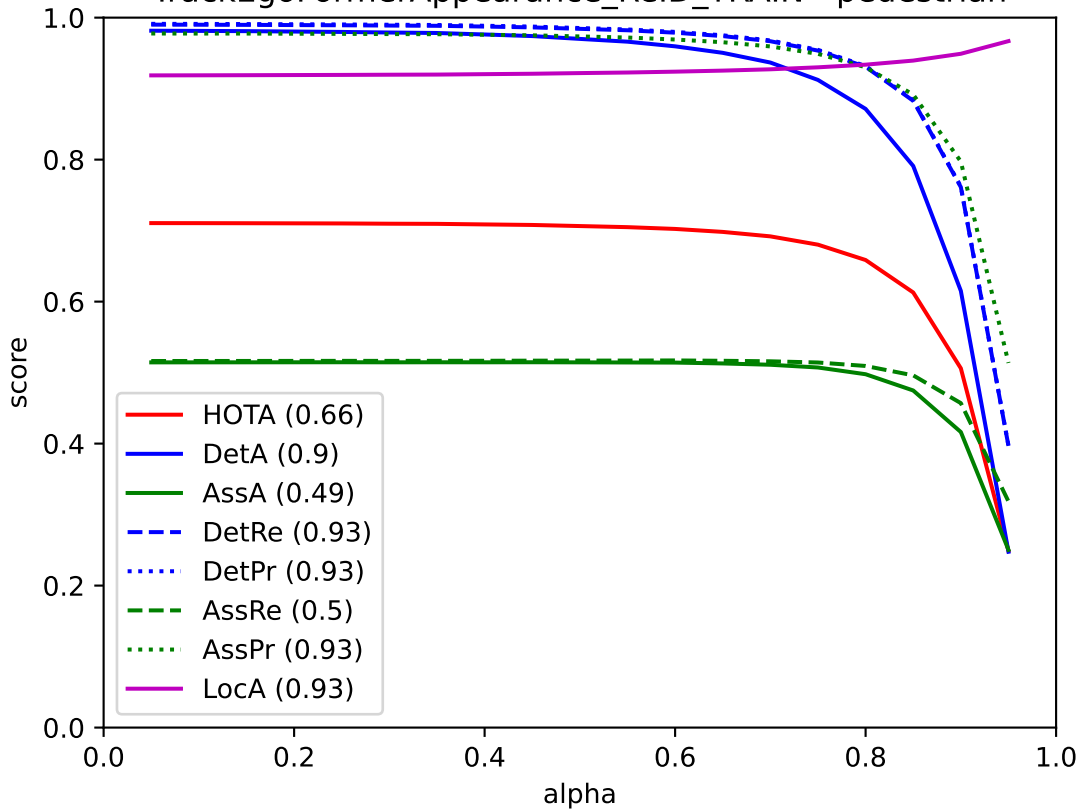
TrackEgoFormerAppearance_ReID_TRAIN - pedestrian
