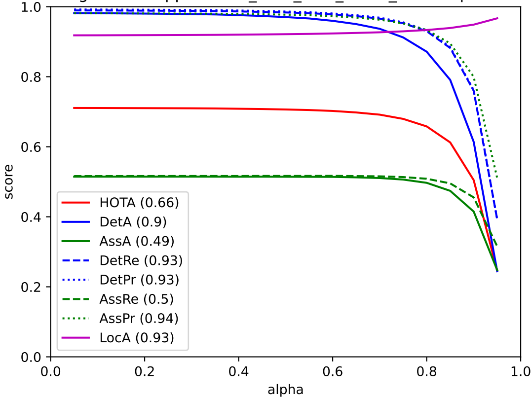
TrackEgoFormerAppearance_ReID_best_MOTA_TRAIN - pedestrian
