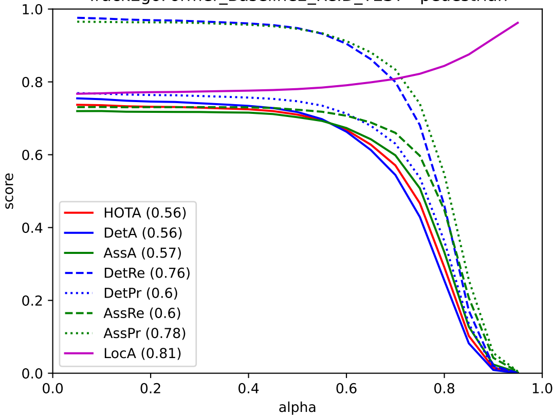
TrackEgoFormer_Baseline2_ReID_TEST - pedestrian
