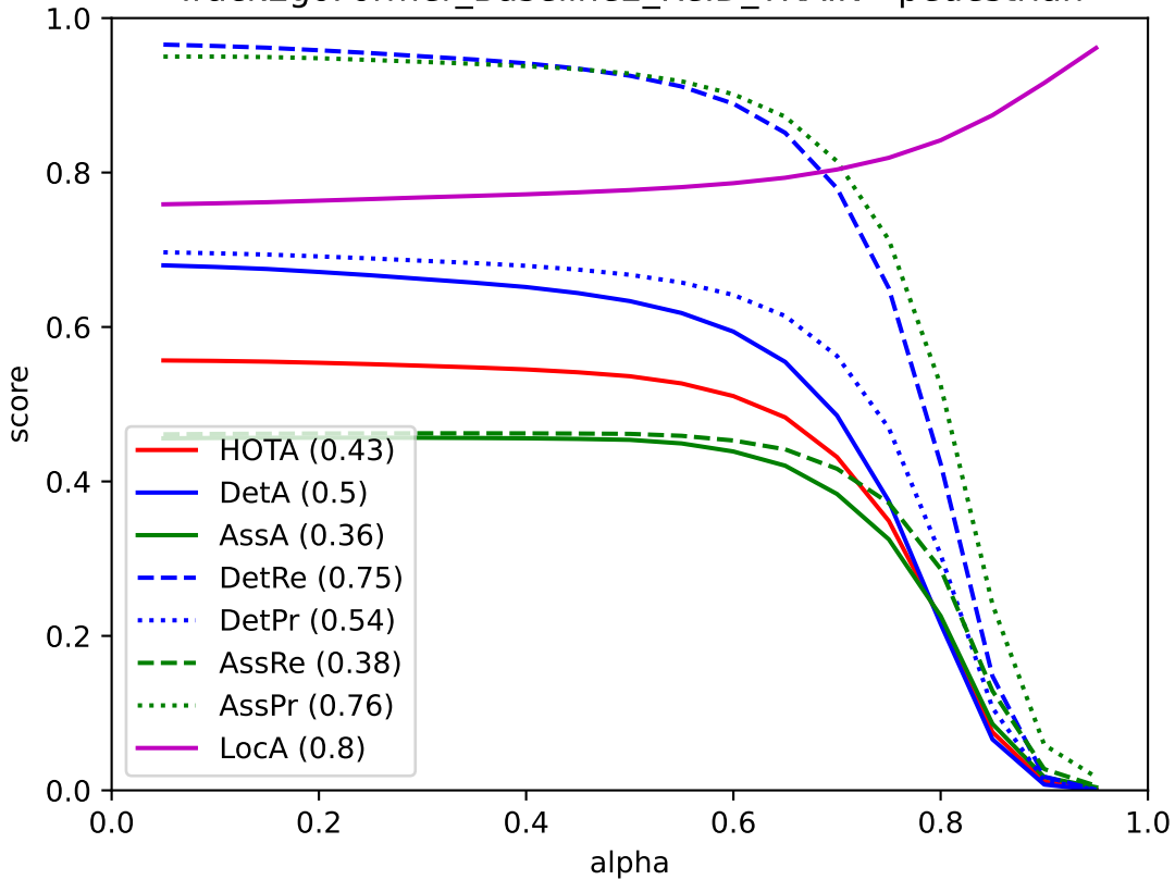
TrackEgoFormer_Baseline2_ReID_TRAIN - pedestrian
