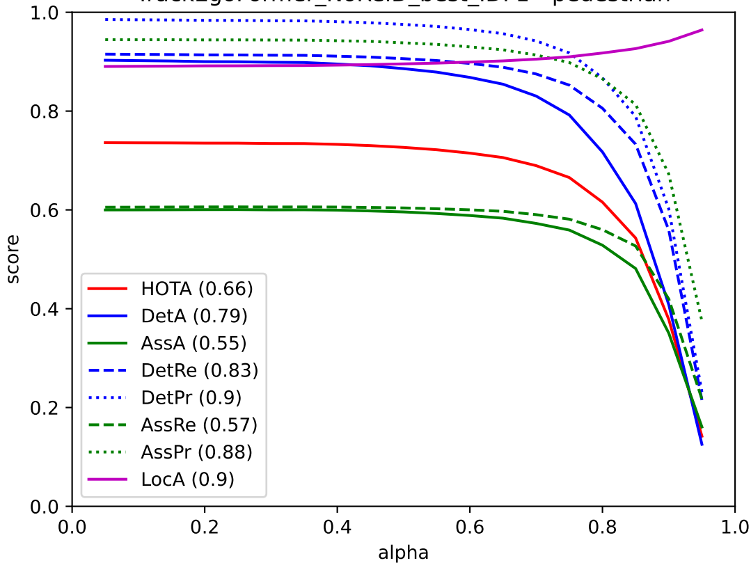
TrackEgoFormer_NoReID_best_IDF1 - pedestrian
