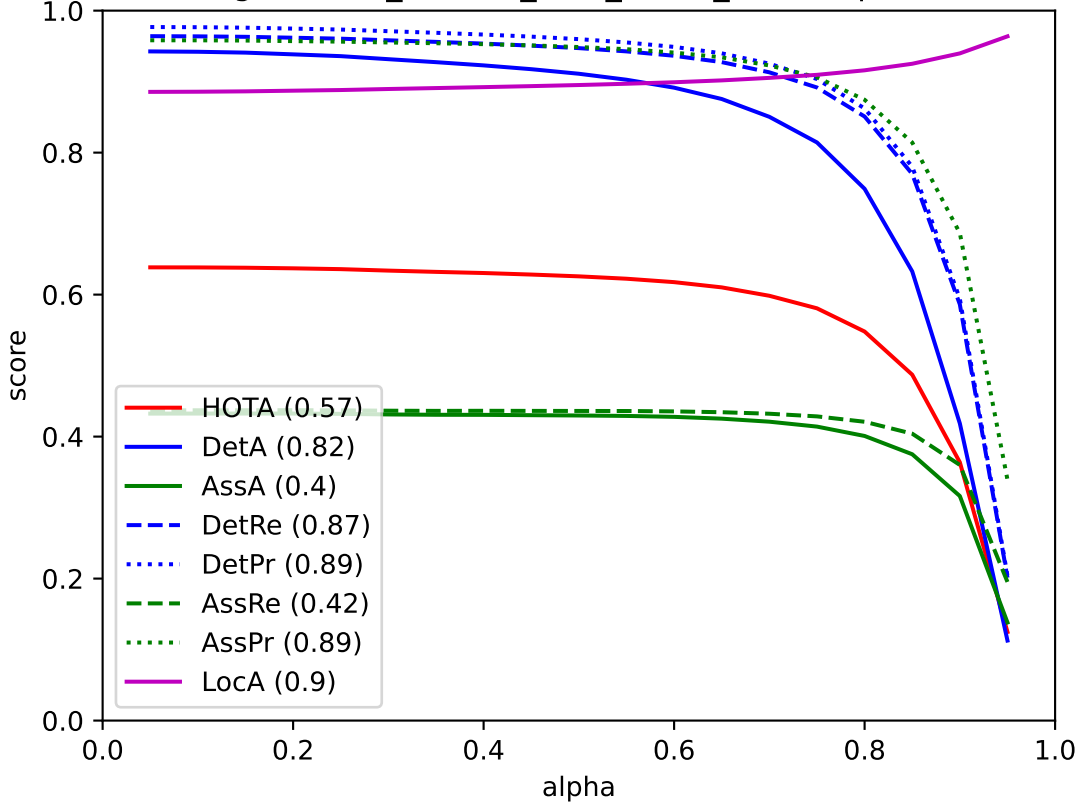
TrackEgoFormer_NoReID_best_MOTA_TRAIN - pedestrian
