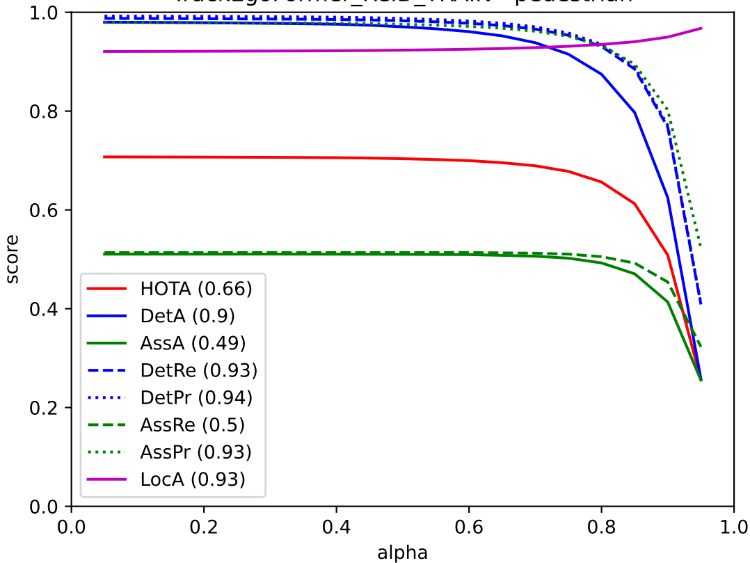
TrackEgoFormer_ReID_TRAIN - pedestrian
