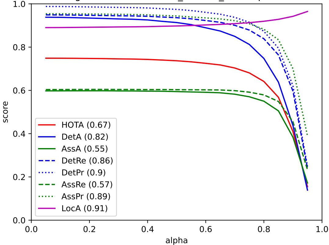
TrackEgoFormerScaleAware_NoReID_TEST - pedestrian
