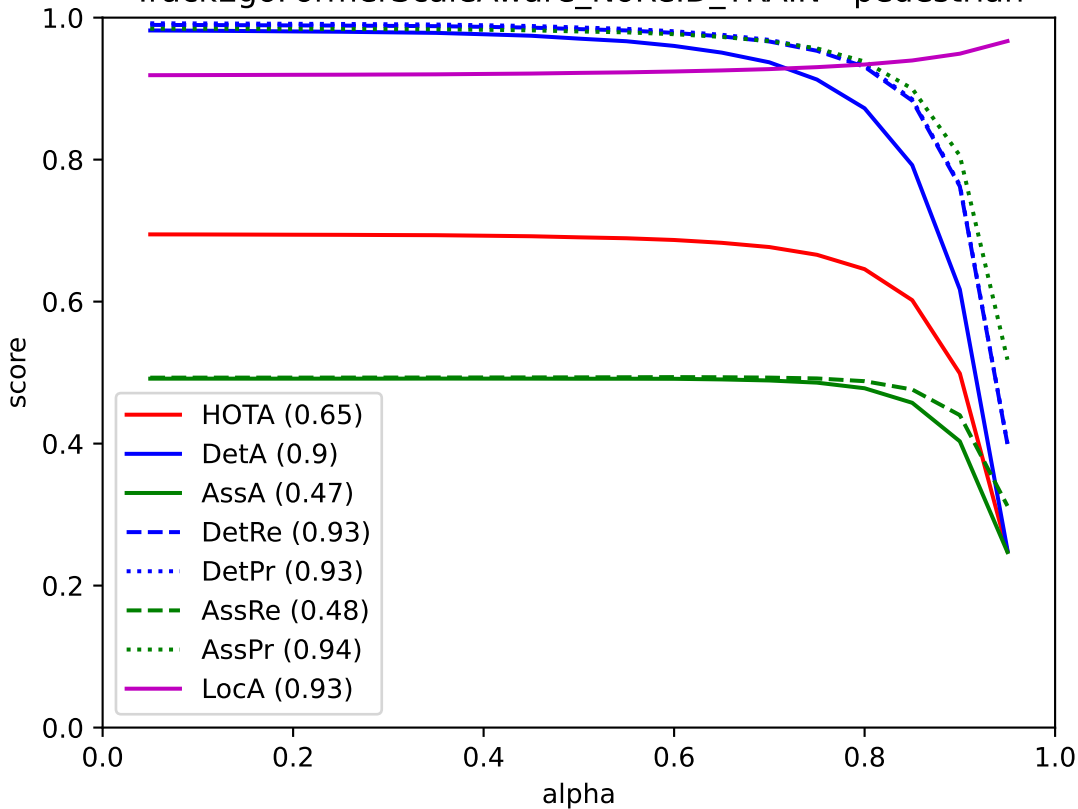
TrackEgoFormerScaleAware_NoReID_TRAIN - pedestrian
