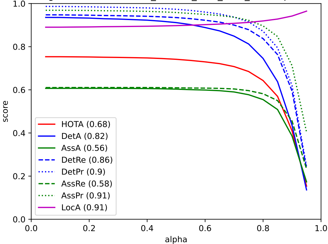
TrackEgoFormerScaleAware_NoReID_best_IDF1_TEST - pedestrian
