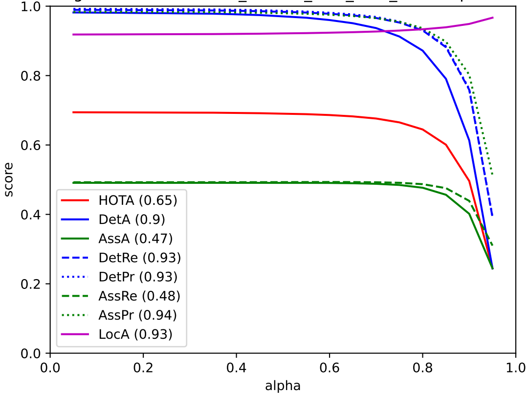
TrackEgoFormerScaleAware_NoReID_best_IDF1_TRAIN - pedestrian
