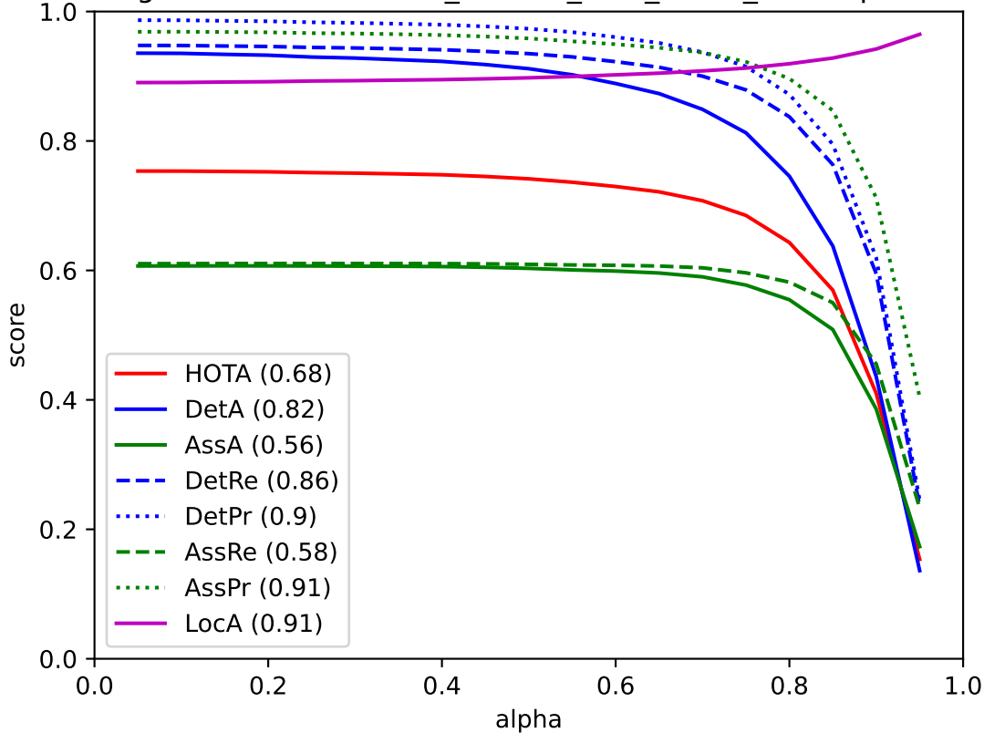
TrackEgoFormerScaleAware_NoReID_best_MOTA_TEST - pedestrian
