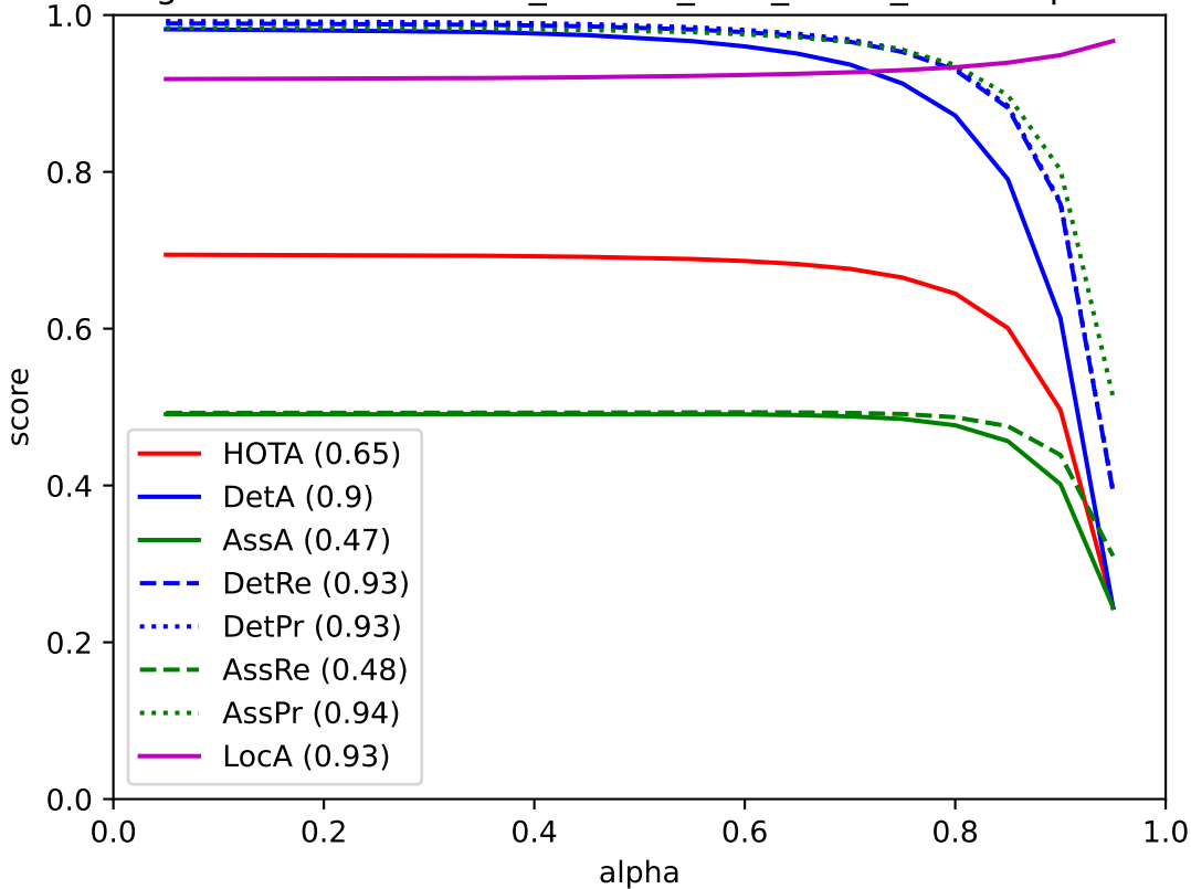
TrackEgoFormerScaleAware_NoReID_best_MOTA_TRAIN - pedestrian
