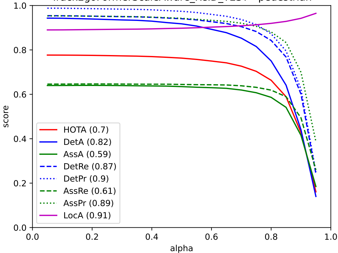
TrackEgoFormerScaleAware_ReID_TEST - pedestrian
