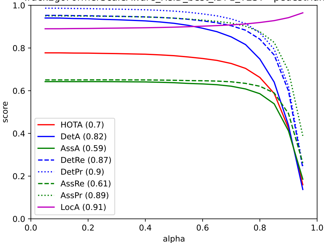
TrackEgoFormerScaleAware_ReID_best_IDF1_TEST - pedestrian
