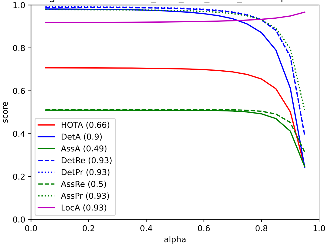
TrackEgoFormerScaleAware_ReID_best_MOTA_TRAIN - pedestrian
